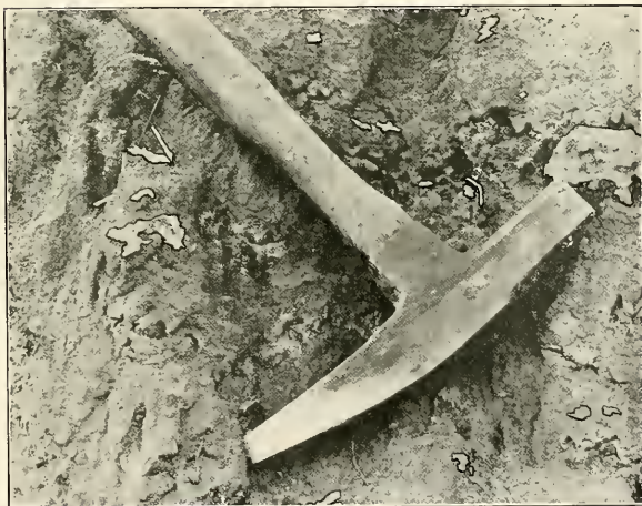
B. Exposure of loess containing concretions. The concretions are outlined by black lines. (Photo by Crane.)
